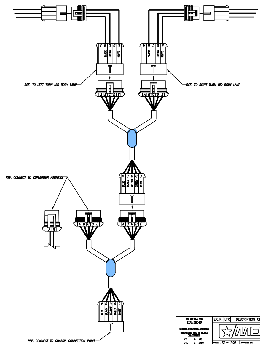
MID BODY TURN LAMPS
